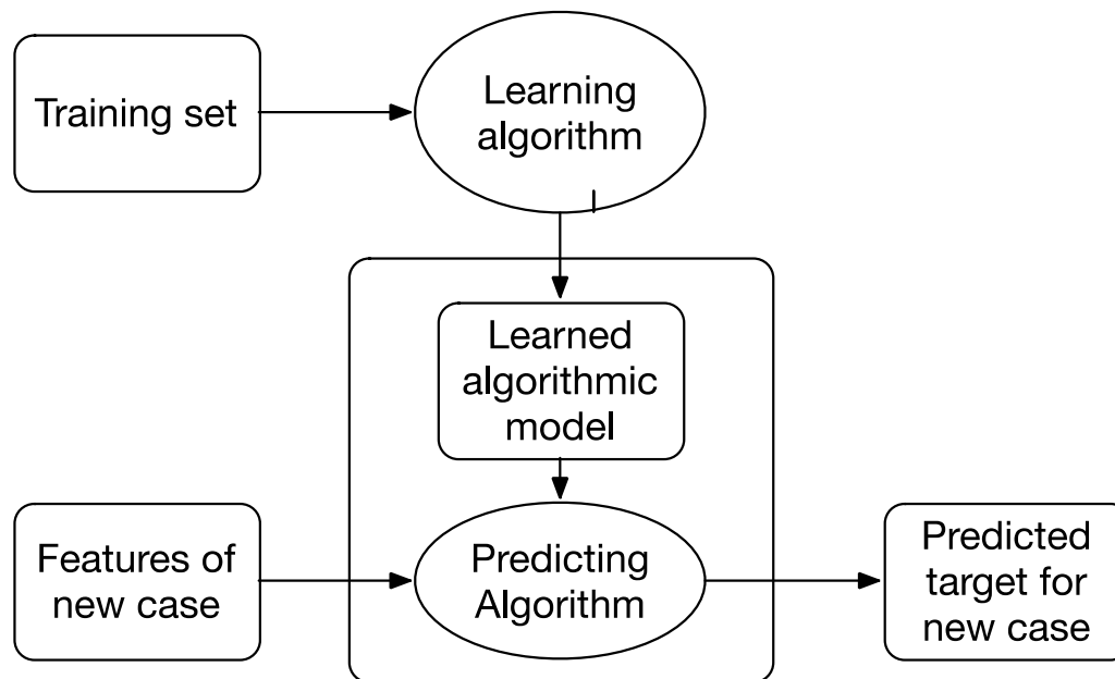
Figure 6 – Supervised learning
